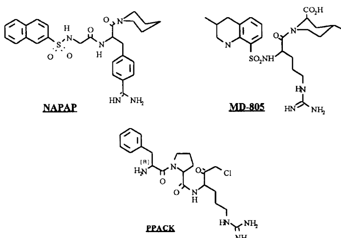
Figure 1. The inhibitors studied: NAPAP , N \alpha -(2-naphthyl-sulfonyl-glycyl)-D-para-amidinophenylalanyl piperidine, K_i = 6.6 nM (racemic form); MD-805 , (2 R ,4 R )-4-methyl-[N \alpha -[(3-methyl-1,2,3,4-tetrahydro-8-quinolyl)sulfonyl]-L-arginyl]-2-piperidine carboxylic acid (also called MQPA, Argipidine or Argatroban, K_i = 39 nM); PPACK , D-Phe-Pro-Arg-CH 2 Cl which binds covalently with K_{inact} = 1.2 \times 10^7 \text{ M}^{-1}\text{S}^{-1} .
