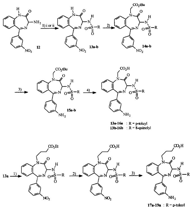
Figure 7. Top: (1) i: \text{NEt}_3 , p -toluylyl- \text{SO}_2\text{Cl} , \text{CHCl}_3 , ii: \text{NEt}_3 , 8-quinolylyl- \text{SO}_2\text{Cl} ; (2) \text{K}_2\text{CO}_3 , \text{BrCH}_2\text{CO}_2t\text{Bu} , DMF; (3) Pd/C, \text{NEt}_3 , \text{HCO}_2\text{H} , \text{CH}_3\text{CN} ; (4) \text{CF}_3\text{CO}_2\text{H} , AcOH. Bottom: (1) KI, \text{BrCH}_2\text{CH}_2\text{CH}_2\text{CO}_2\text{Et} , DMF; (2) 1 N NaOH, EtOH; (3) Pd/C, \text{H}_2 , MeOH.
