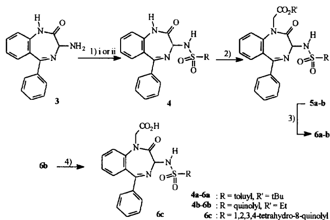
Figure 5. (1) i: NEt 3 , p -toluyl-SO 2 Cl, CHCl 3 , ii: 8-quinolyl-SO 2 Cl; (2) NaH, BrCH 2 CO 2 tBu, DMF to get 5a or NaH, BrCH 2 CO 2 Et, DMF to obtain 5b ; (3) 1 N NaOH, MeOH for 6b or HCO 2 H, 70 °C for 6a ; (4) Pd/C, H 2 , MeOH.
